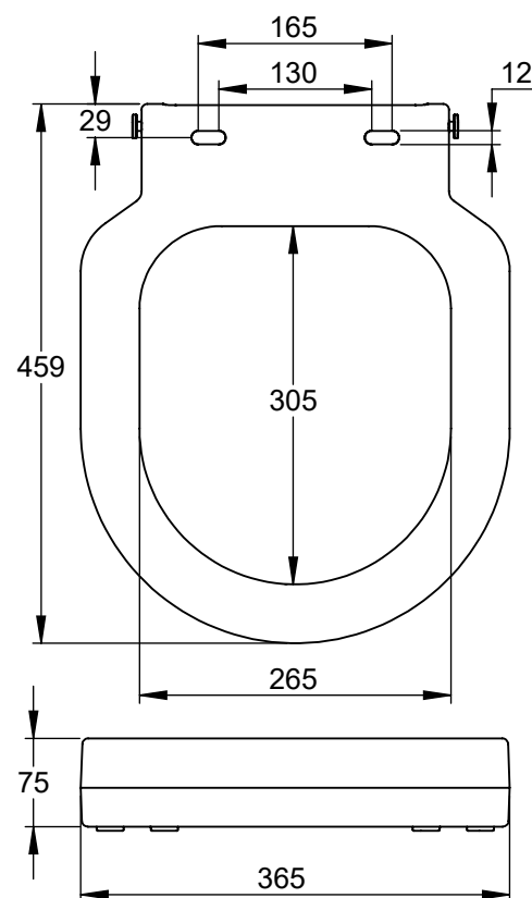
66494 ASHBY LIFT D-SHAPE
