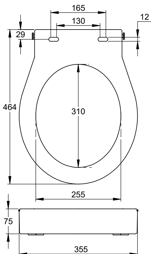
66294 ASHBY LIFT OVAL
